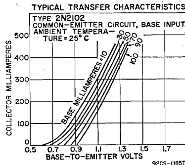
Figure 25. Transfer-characteristic curves.
