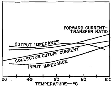
Figure 120. Variation of transistor characteristics with temperature.
