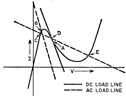
Figure 110. Typical load lines for tunnel-diode circuits.
