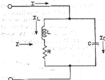
Figure 50. Simple parallel resonant circuit.
