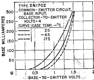
TYPICAL BASE CHARACTERISTICS
