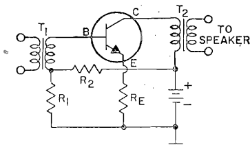
Figure 43. Class A power-amplifier circuit.
