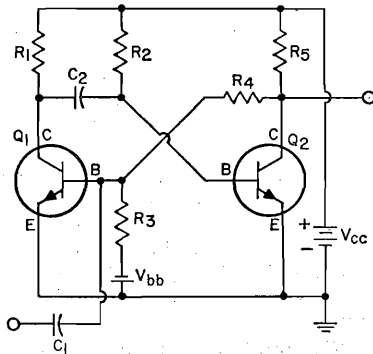
Figure 76. Monostable multivibrator.
