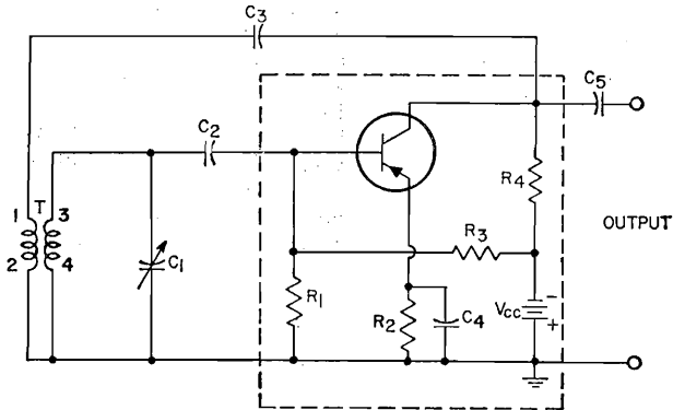
Figure 64. Tuned-base oscillator.
