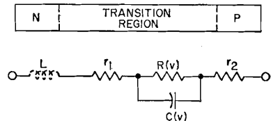
Figure 108. Equivalent circuit for a tunnel diode.
