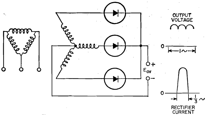
Figure 89. Three-phase (Y) half-wave circuit.
