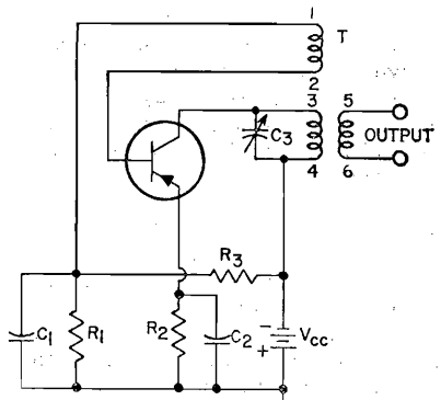
Figure 65. Tuned-collector oscillator.
