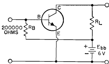
Figure 30. "Fixed-bias" arrangement for common-emitter circuit.
