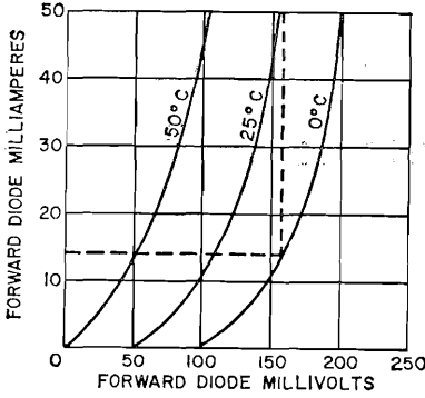
Figure 119. Forward characteristics of compensating diode.
