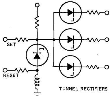
Figure 115. Logic circuit using a tunnel diode and three tunnel rectifiers.
