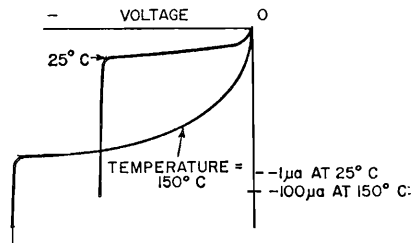
Figure 81. Typical reverse characteristics.
